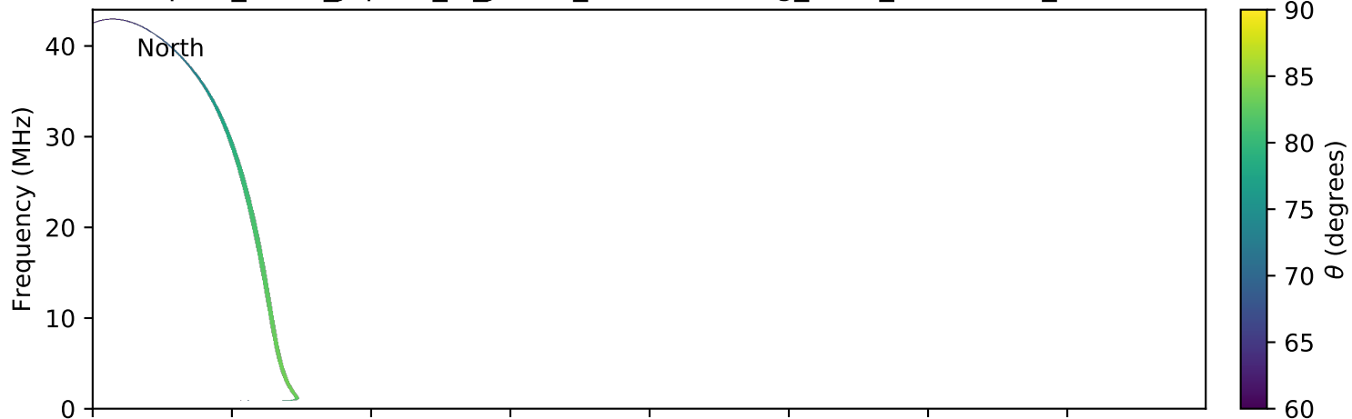
expres_earth_jupiter_io_jrm09_lossc-wid1deg_3kev_20060703_v01.cdf
