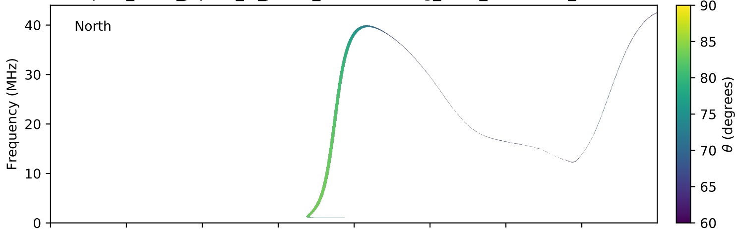
expres_earth_jupiter_io_jrm09_lossc-wid1deg_3kev_20060702_v01.cdf
