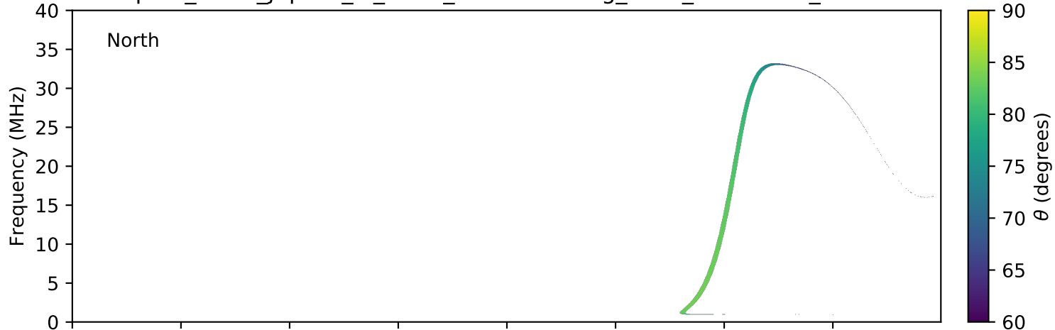
expres_earth_jupiter_io_isaac_lossc-wid1deg_3kev_20060730_v01.cdf
