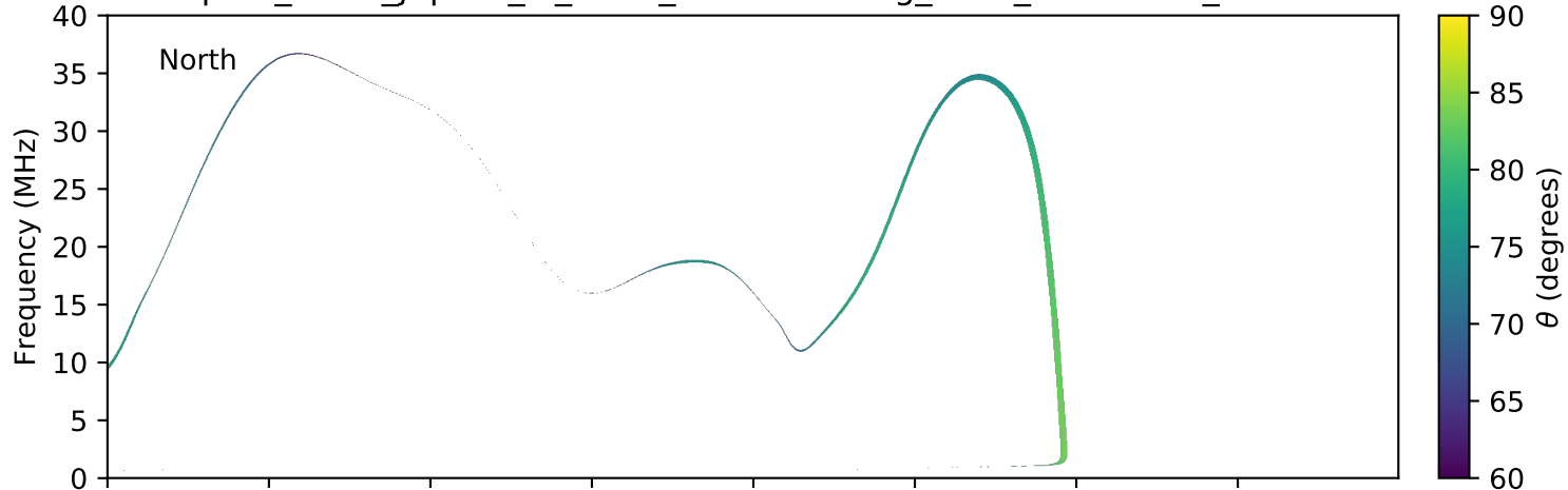
expres_earth_jupiter_io_isaac_lossc-wid1deg_3kev_20060729_v01.cdf
