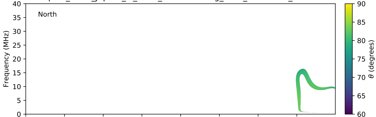
expres_earth_jupiter_io_isaac_lossc-wid1deg_3kev_20060728_v01.cdf
