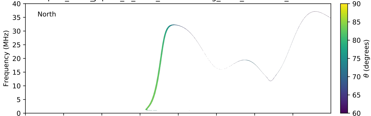
expres_earth_jupiter_io_isaac_lossc-wid1deg_3kev_20060725_v01.cdf
