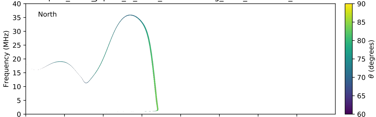
expres_earth_jupiter_io_isaac_lossc-wid1deg_3kev_20060724_v01.cdf
