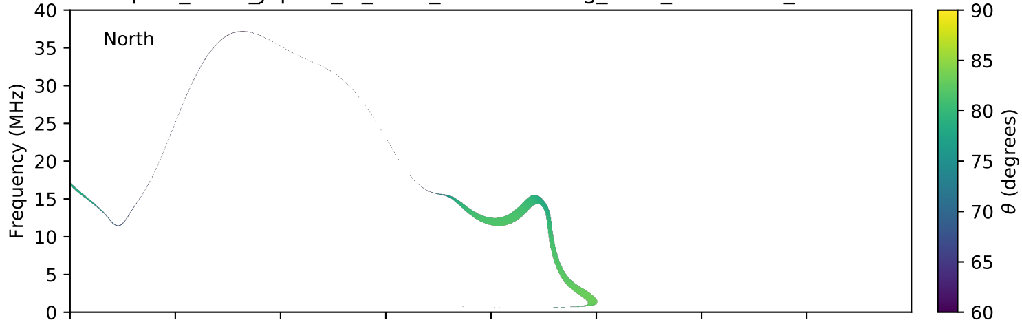
expres_earth_jupiter_io_isaac_lossc-wid1deg_3kev_20060722_v01.cdf
