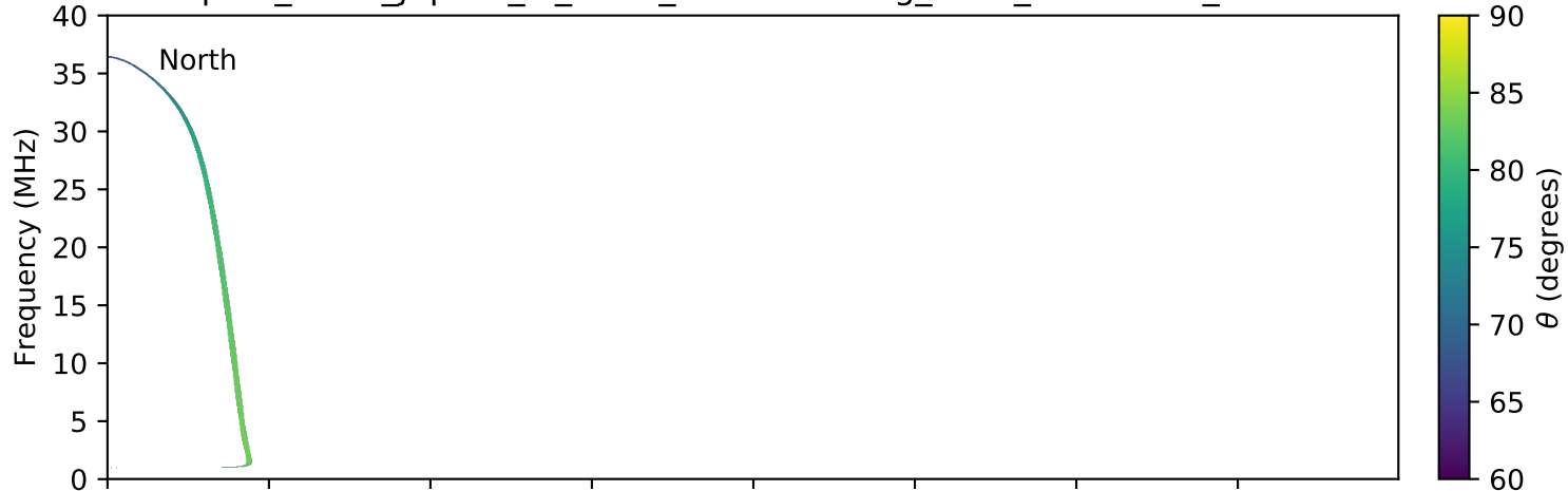
expres_earth_jupiter_io_isaac_lossc-wid1deg_3kev_20060719_v01.cdf
