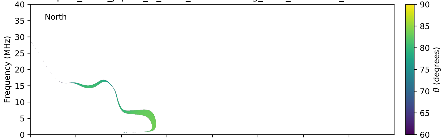
expres_earth_jupiter_io_isaac_lossc-wid1deg_3kev_20060717_v01.cdf
