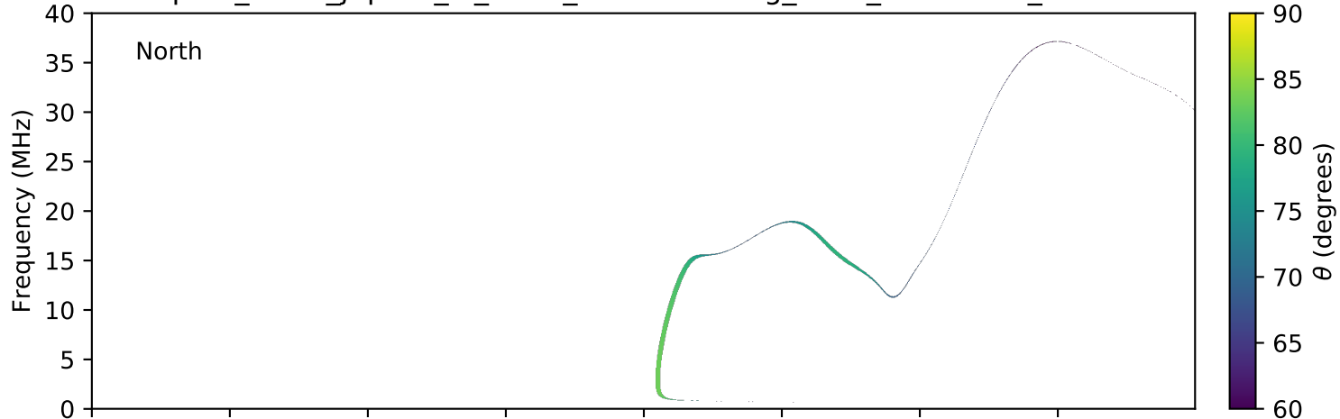
expres_earth_jupiter_io_isaac_lossc-wid1deg_3kev_20060716_v01.cdf
