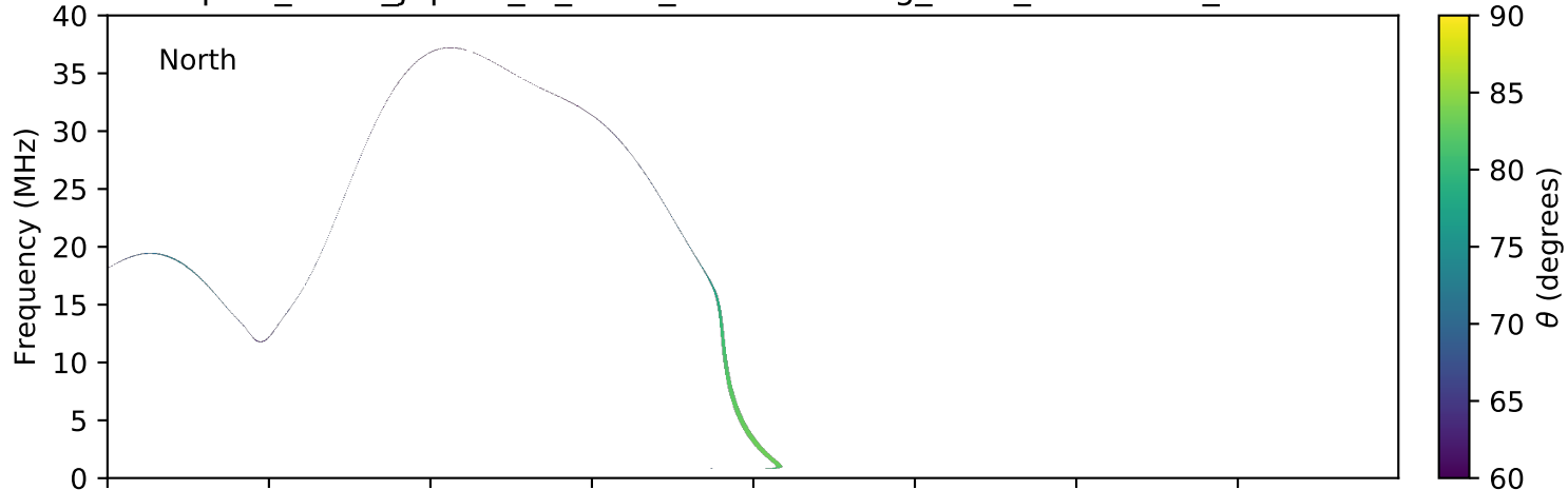
expres_earth_jupiter_io_isaac_lossc-wid1deg_3kev_20060715_v01.cdf
