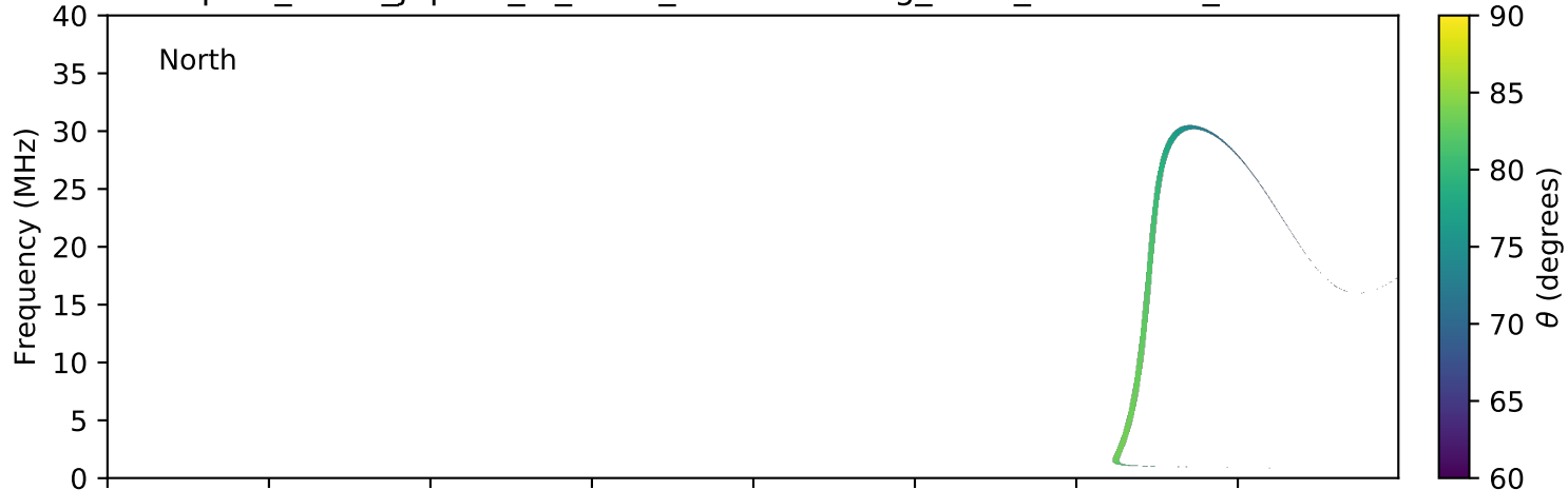
expres_earth_jupiter_io_isaac_lossc-wid1deg_3kev_20060714_v01.cdf
