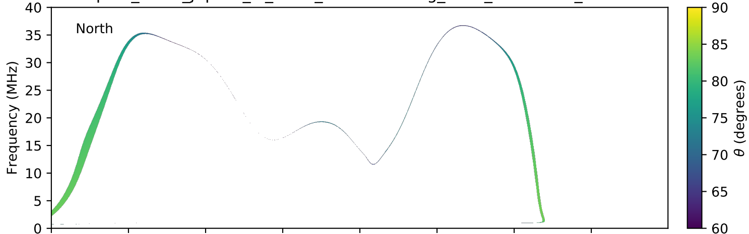
expres_earth_jupiter_io_isaac_lossc-wid1deg_3kev_20060713_v01.cdf
