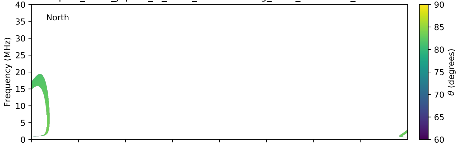
expres_earth_jupiter_io_isaac_lossc-wid1deg_3kev_20060712_v01.cdf
