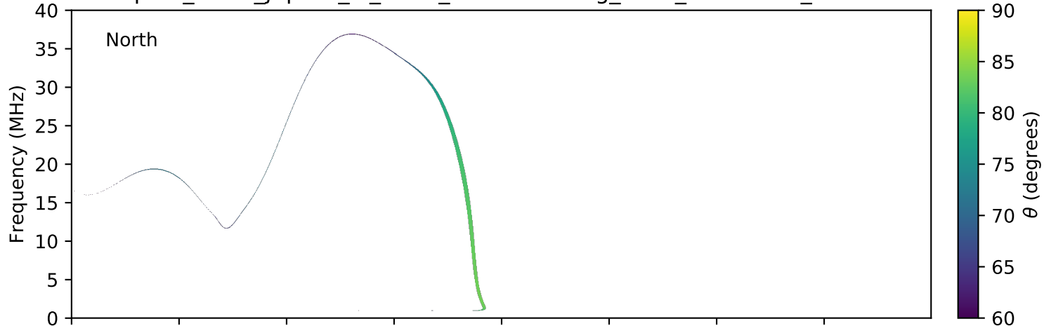
expres_earth_jupiter_io_isaac_lossc-wid1deg_3kev_20060708_v01.cdf
