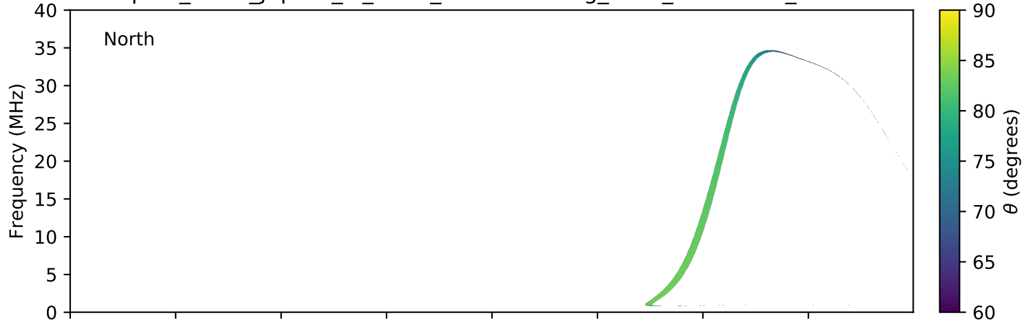
expres_earth_jupiter_io_isaac_lossc-wid1deg_3kev_20060707_v01.cdf
