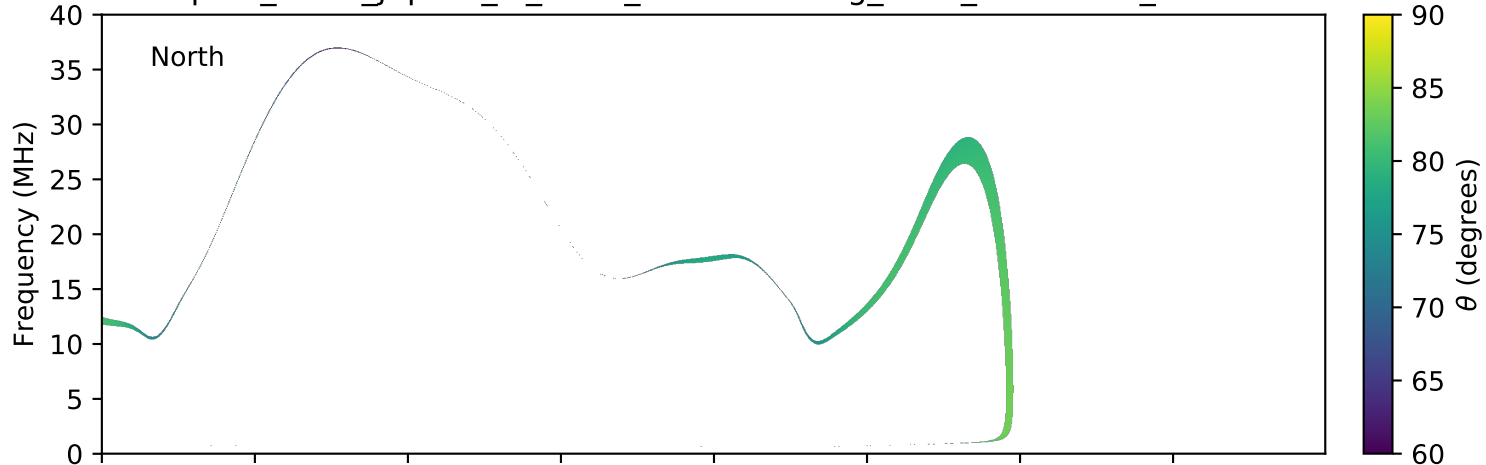
expres_earth_jupiter_io_isaac_lossc-wid1deg_3kev_20060706_v01.cdf
