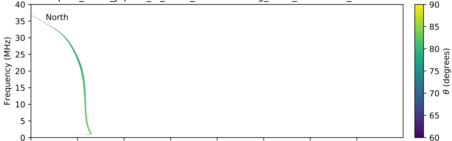
expres_earth_jupiter_io_isaac_lossc-wid1deg_3kev_20060703_v01.cdf
