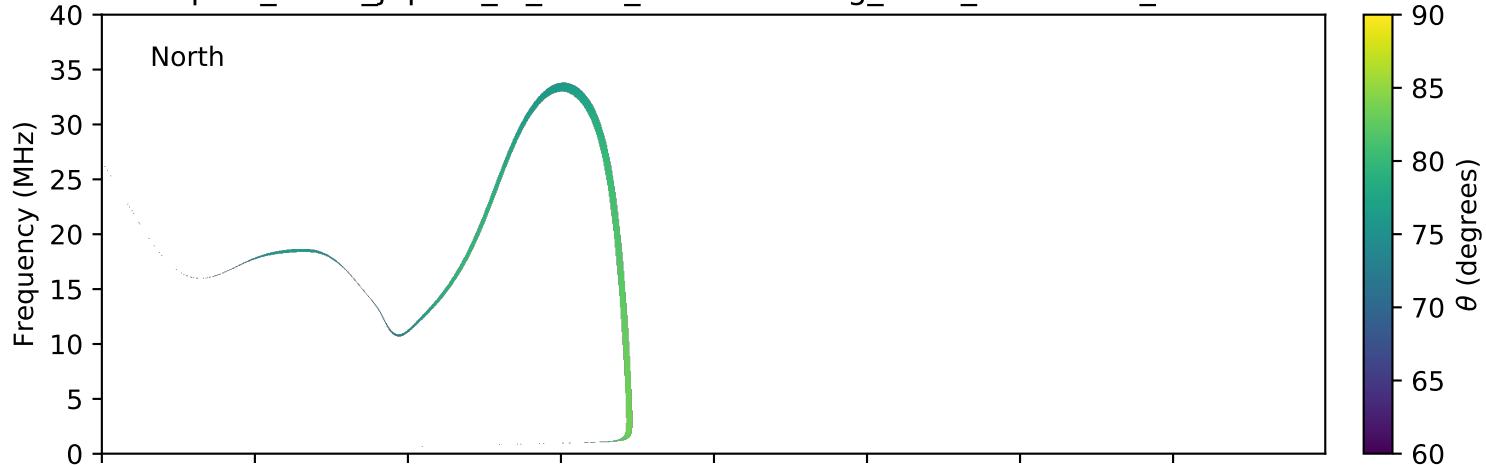
expres_earth_jupiter_io_isaac_lossc-wid1deg_3kev_20060701_v01.cdf
