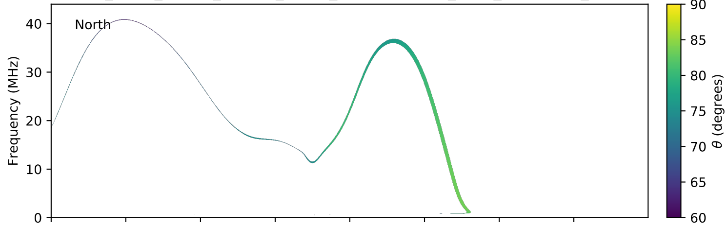
expres_earth_jupiter_europa_jrm09_lossc-wid1deg_3kev_20060731_v01.cdf
