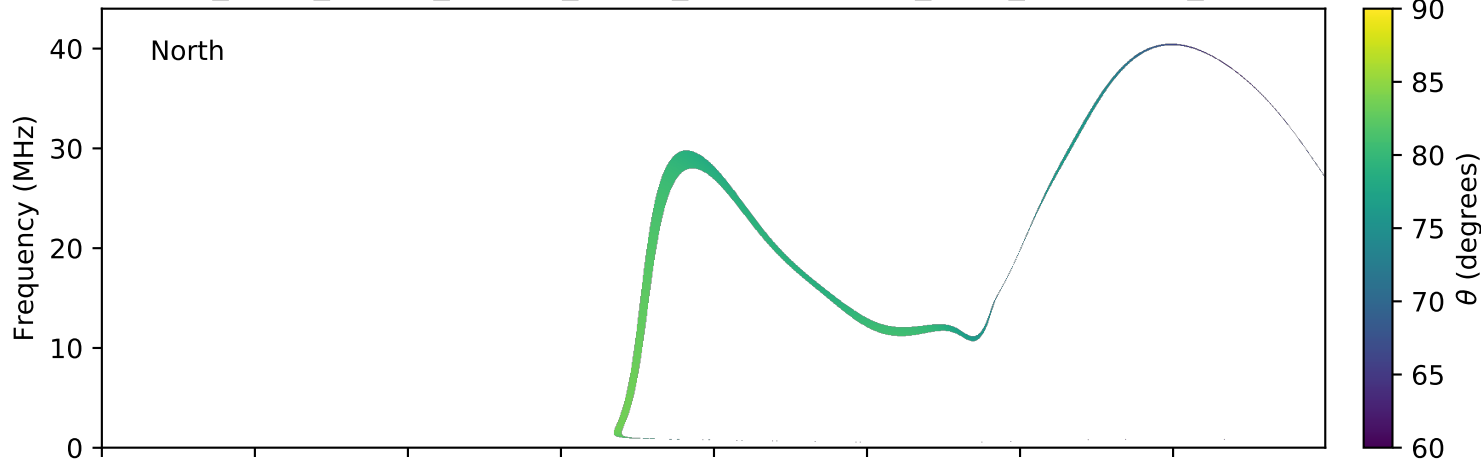
expres_earth_jupiter_europa_jrm09_lossc-wid1deg_3kev_20060712_v01.cdf
