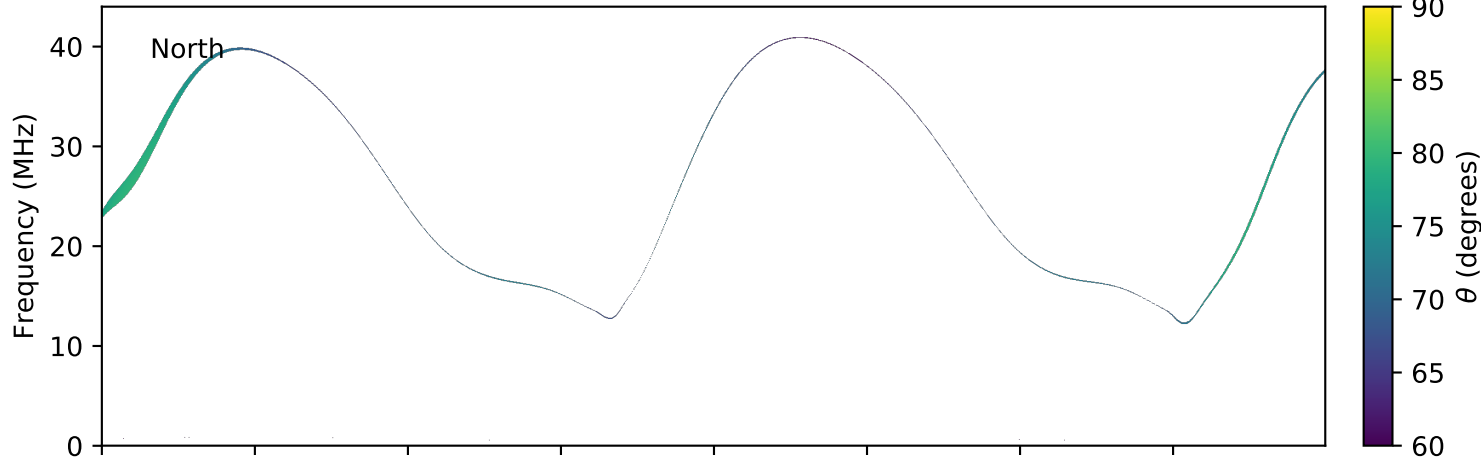
expres_earth_jupiter_europa_jrm09_lossc-wid1deg_3kev_20060702_v01.cdf
