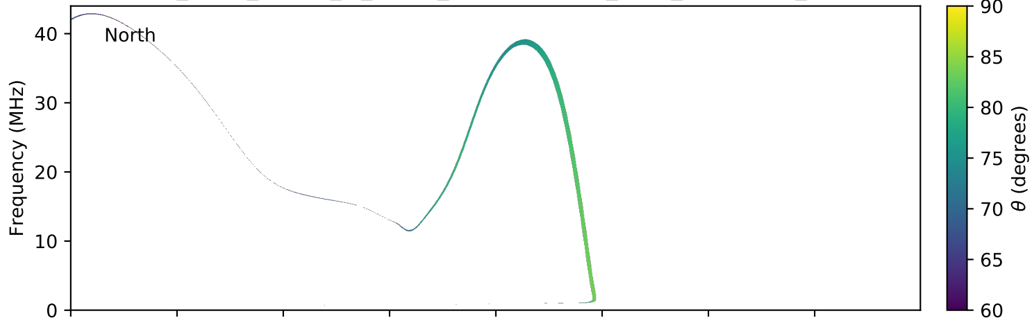
expres_earth_jupiter_io_jrm09_lossc-wid1deg_3kev_20060530_v01.cdf
