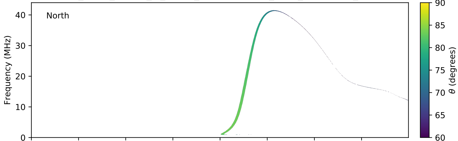
expres_earth_jupiter_io_jrm09_lossc-wid1deg_3kev_20060524_v01.cdf
