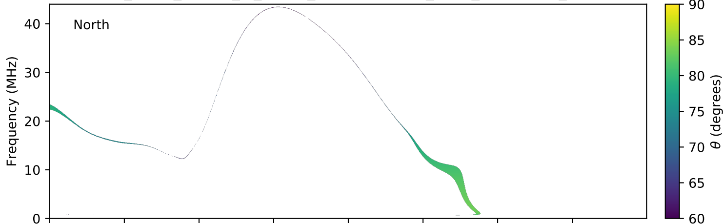
expres_earth_jupiter_io_jrm09_lossc-wid1deg_3kev_20060521_v01.cdf
