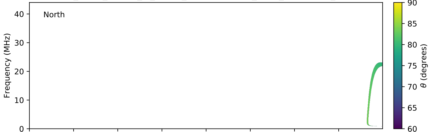
expres_earth_jupiter_io_jrm09_lossc-wid1deg_3kev_20060520_v01.cdf
