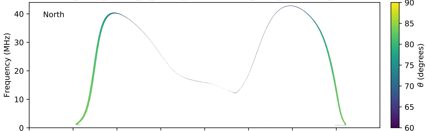
expres_earth_jupiter_io_jrm09_lossc-wid1deg_3kev_20060512_v01.cdf
