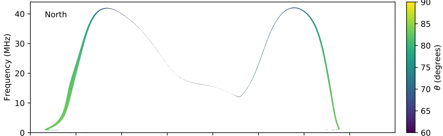
expres_earth_jupiter_io_jrm09_lossc-wid1deg_3kev_20060505_v01.cdf
