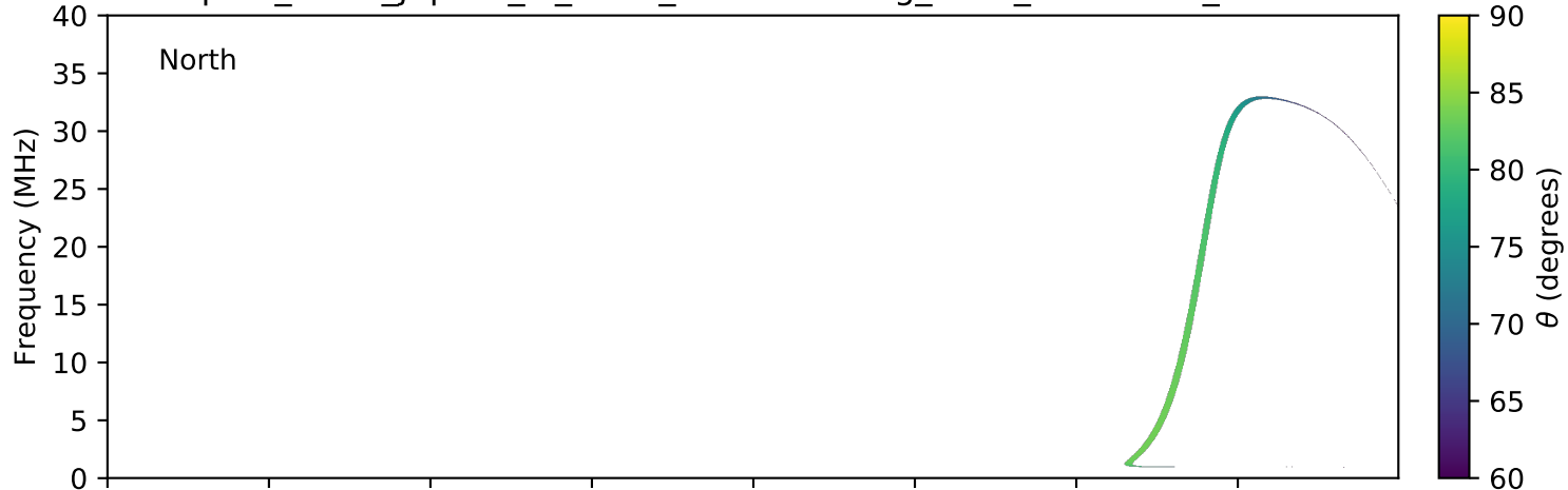
expres_earth_jupiter_io_isaac_lossc-wid1deg_3kev_20060529_v01.cdf
