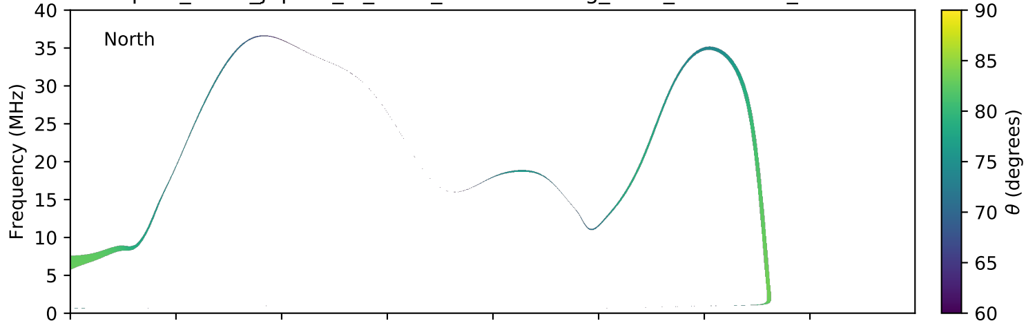
expres_earth_jupiter_io_isaac_lossc-wid1deg_3kev_20060528_v01.cdf
