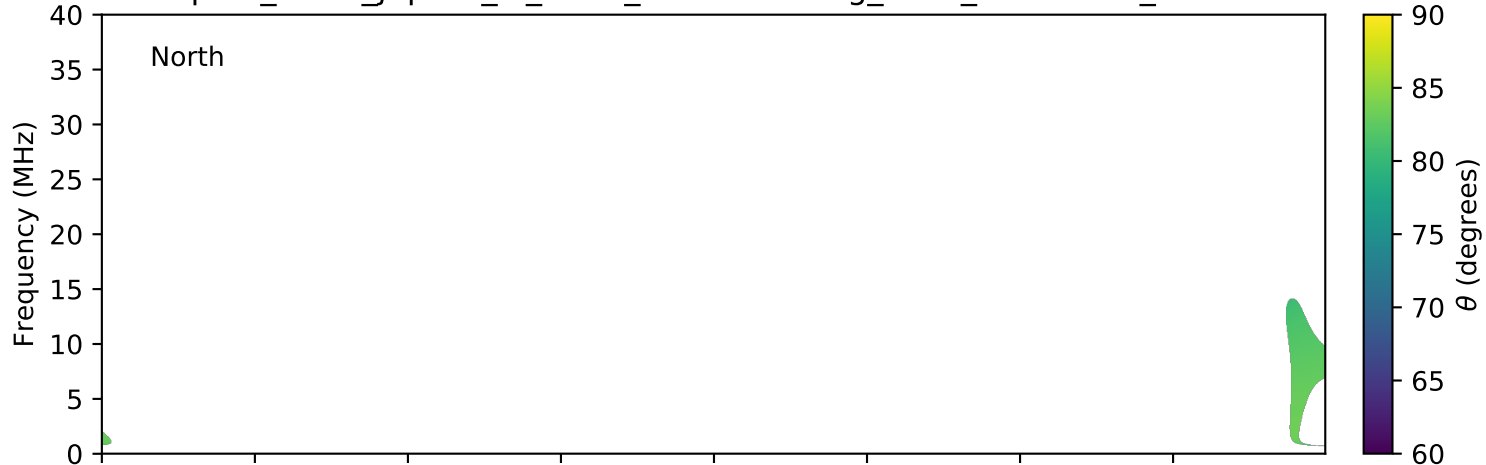
expres_earth_jupiter_io_isaac_lossc-wid1deg_3kev_20060527_v01.cdf
