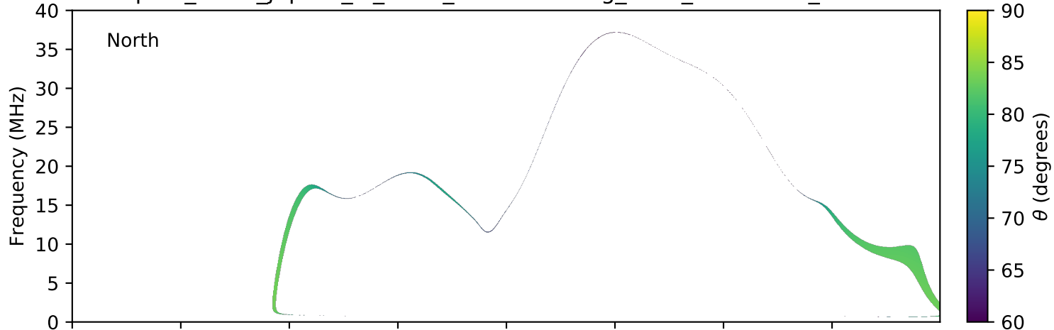
expres_earth_jupiter_io_isaac_lossc-wid1deg_3kev_20060526_v01.cdf
