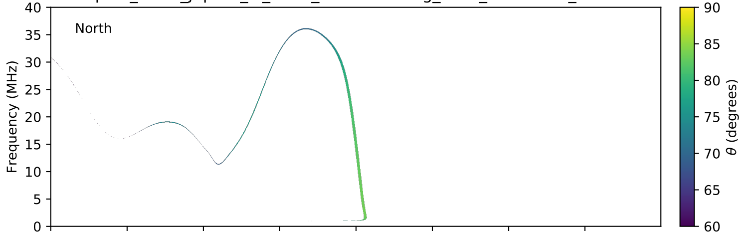
expres_earth_jupiter_io_isaac_lossc-wid1deg_3kev_20060523_v01.cdf
