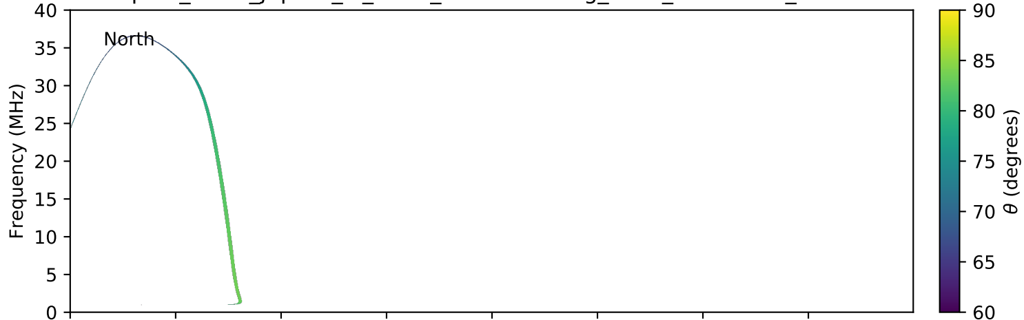
expres_earth_jupiter_io_isaac_lossc-wid1deg_3kev_20060518_v01.cdf
