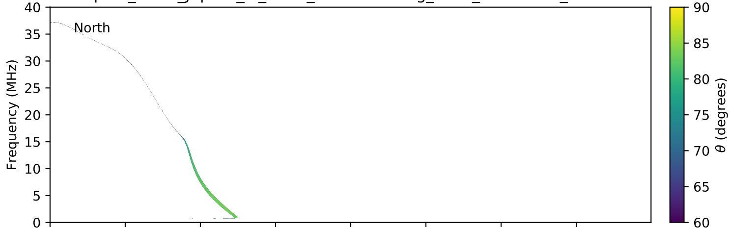
expres_earth_jupiter_io_isaac_lossc-wid1deg_3kev_20060509_v01.cdf
