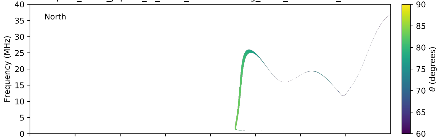
expres_earth_jupiter_io_isaac_lossc-wid1deg_3kev_20060508_v01.cdf
