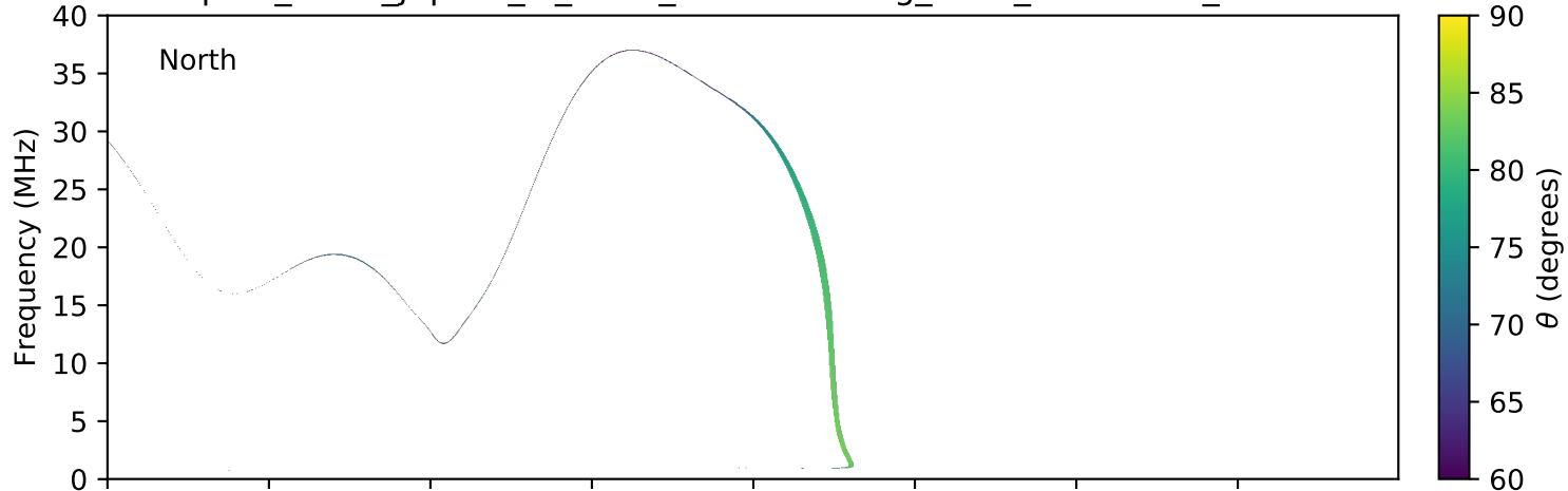
expres_earth_jupiter_io_isaac_lossc-wid1deg_3kev_20060507_v01.cdf
