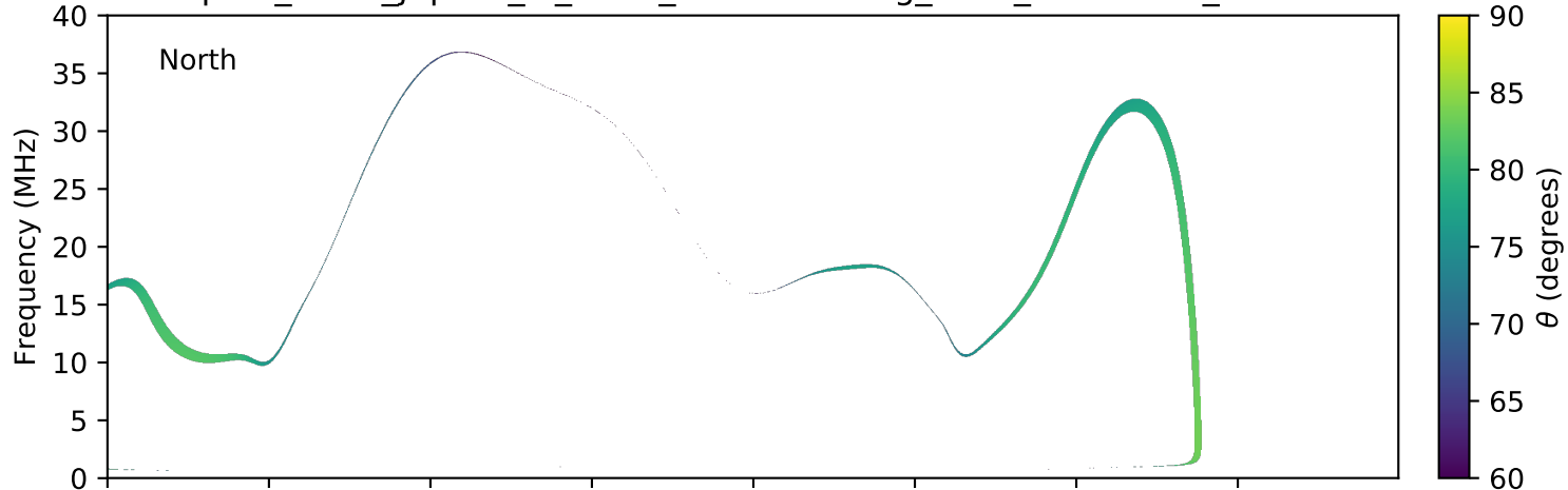
expres_earth_jupiter_io_isaac_lossc-wid1deg_3kev_20060505_v01.cdf
