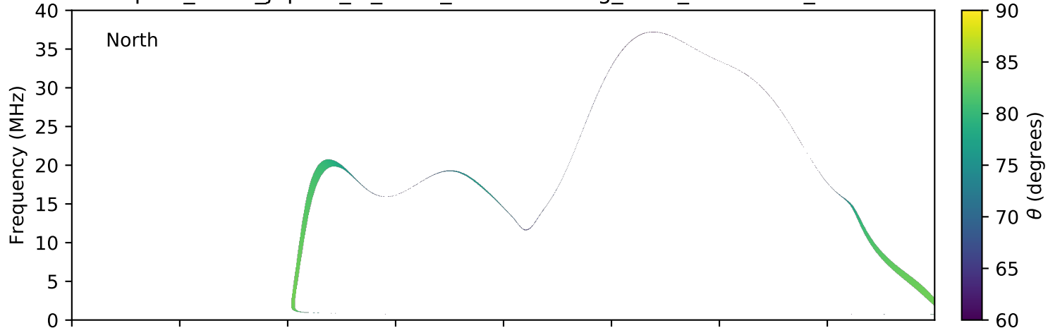
expres_earth_jupiter_io_isaac_lossc-wid1deg_3kev_20060503_v01.cdf
