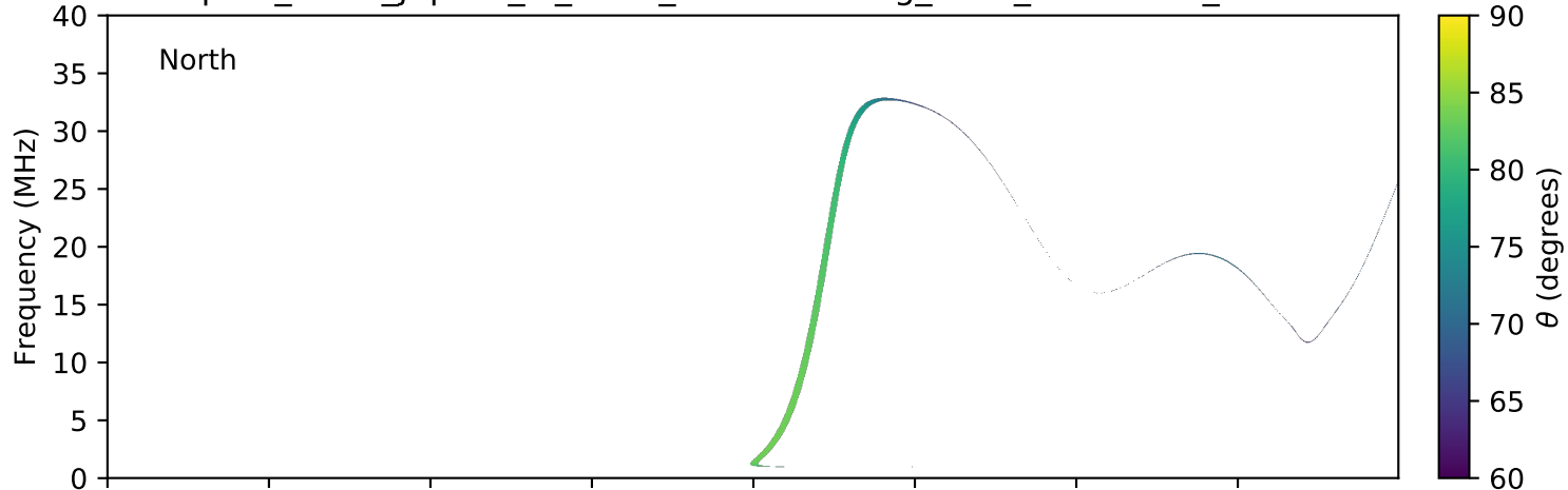
expres_earth_jupiter_io_isaac_lossc-wid1deg_3kev_20060501_v01.cdf
