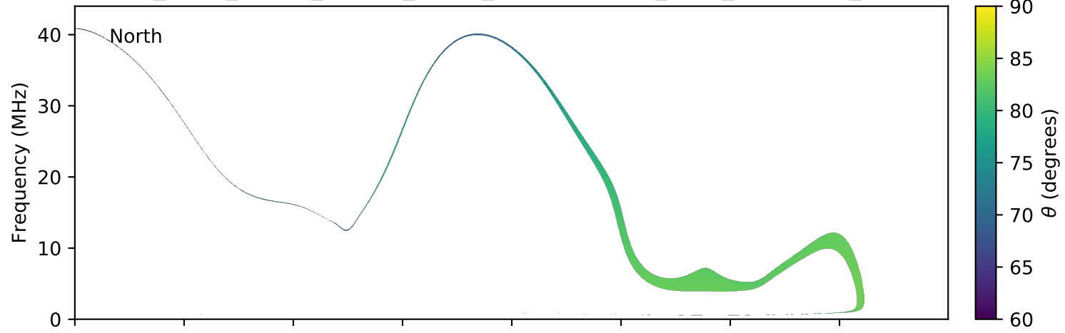
expres_earth_jupiter_europa_jrm09_lossc-wid1deg_3kev_20060528_v01.cdf
