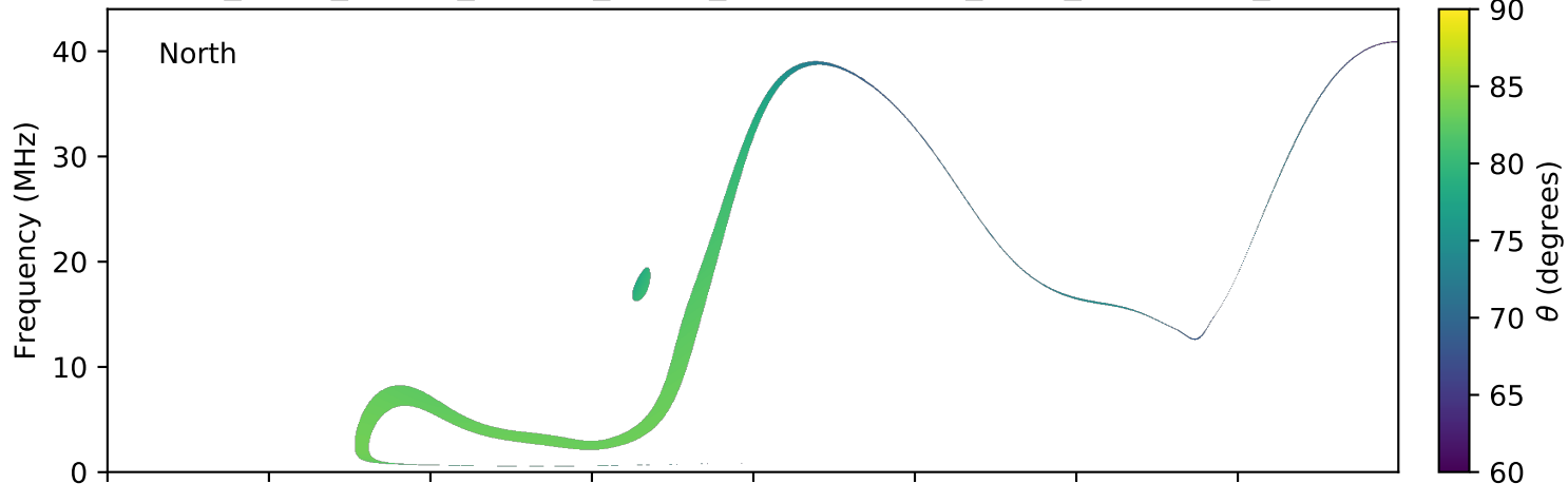
expres_earth_jupiter_europa_jrm09_lossc-wid1deg_3kev_20060527_v01.cdf
