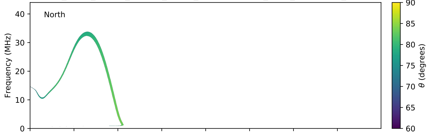
expres_earth_jupiter_europa_jrm09_lossc-wid1deg_3kev_20060525_v01.cdf
