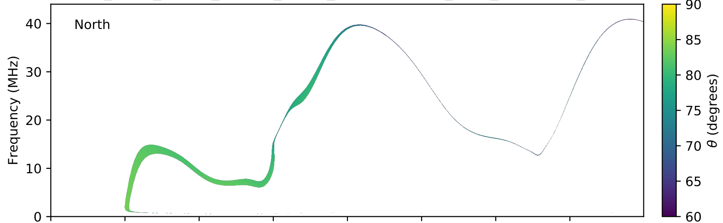
expres_earth_jupiter_europa_jrm09_lossc-wid1deg_3kev_20060520_v01.cdf
