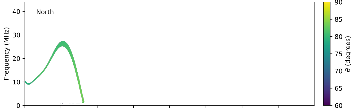
expres_earth_jupiter_europa_jrm09_lossc-wid1deg_3kev_20060518_v01.cdf
