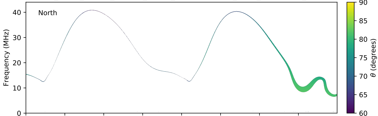
expres_earth_jupiter_europa_jrm09_lossc-wid1deg_3kev_20060510_v01.cdf
