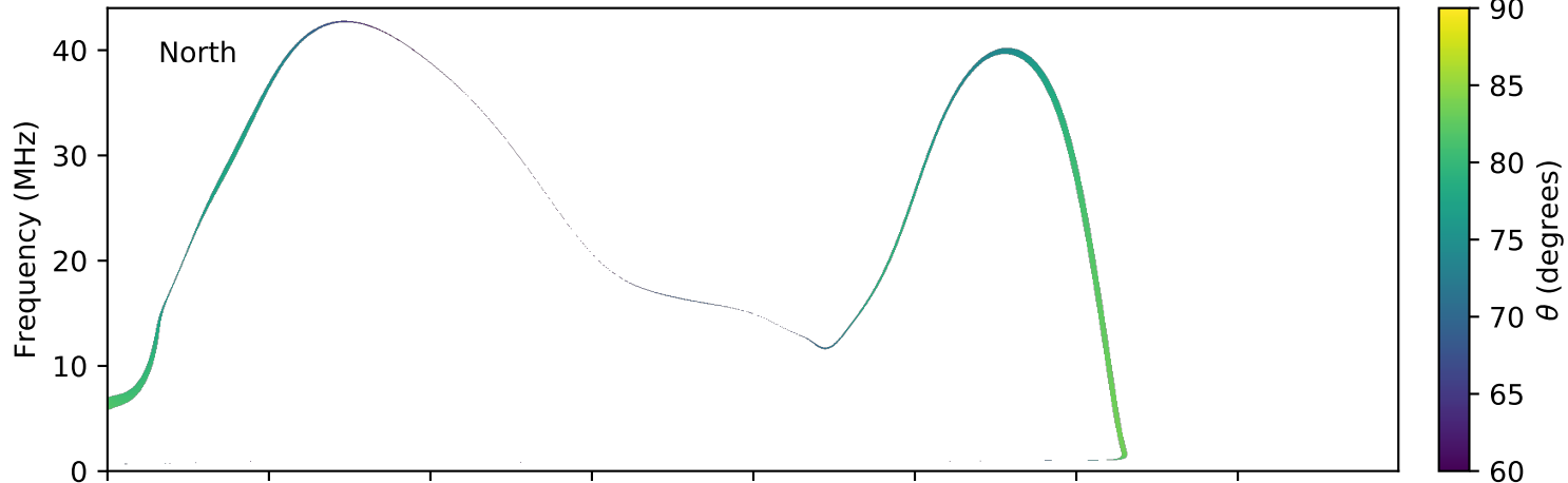
expres_earth_jupiter_io_jrm09_lossc-wid1deg_3kev_20060428_v01.cdf
