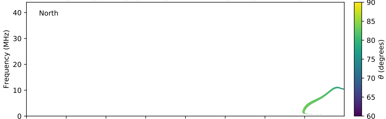
expres_earth_jupiter_io_jrm09_lossc-wid1deg_3kev_20060420_v01.cdf
