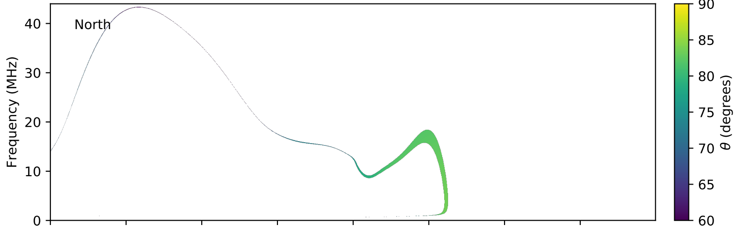
expres_earth_jupiter_io_jrm09_lossc-wid1deg_3kev_20060414_v01.cdf
